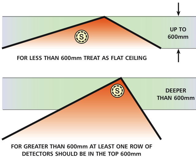
Smoke detector under pitched roofs
