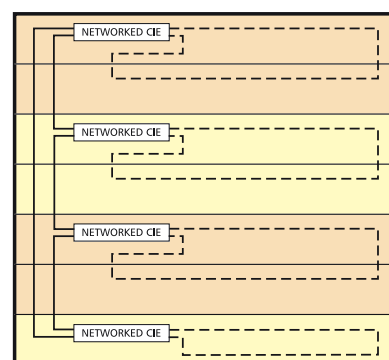
Standard Fire Resisting Cable
