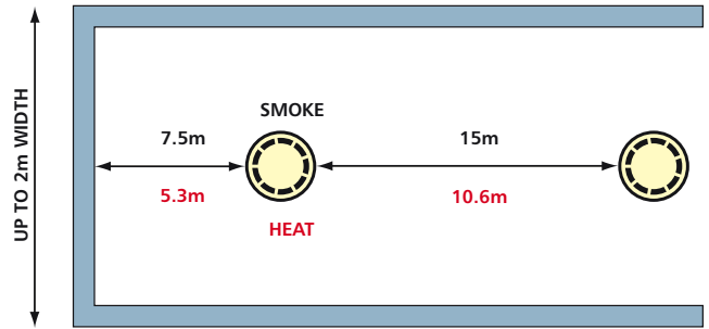
Smoke & Heat detector spacing in corridors (category P only)
