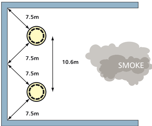
Smoke detector spacing (under flat horizontal ceiling)
