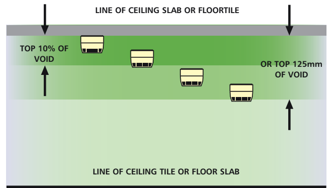
Mounting detectors in voids
